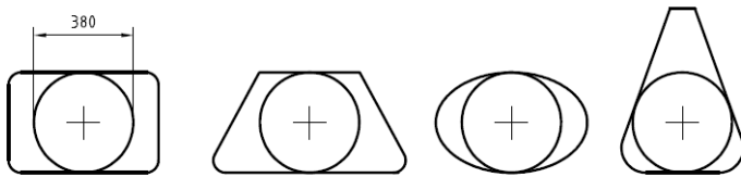
Figure 1 — Measurement of minimum clear opening
